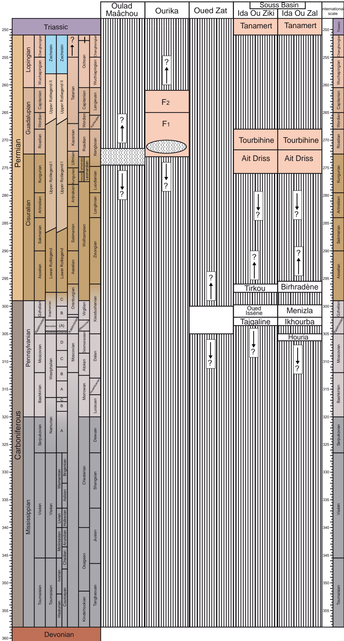
Geological stratigraphic column showing Permian, Carboniferous, and Triassic stages across various basins: Oulad Maâchou, Ourika, Oued Zat, and Souss Basin (Ida Ou Ziki, Ida Ou Zal).
